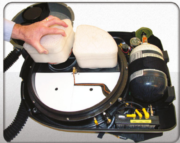
New disposable, Solid Core Scrubber®
